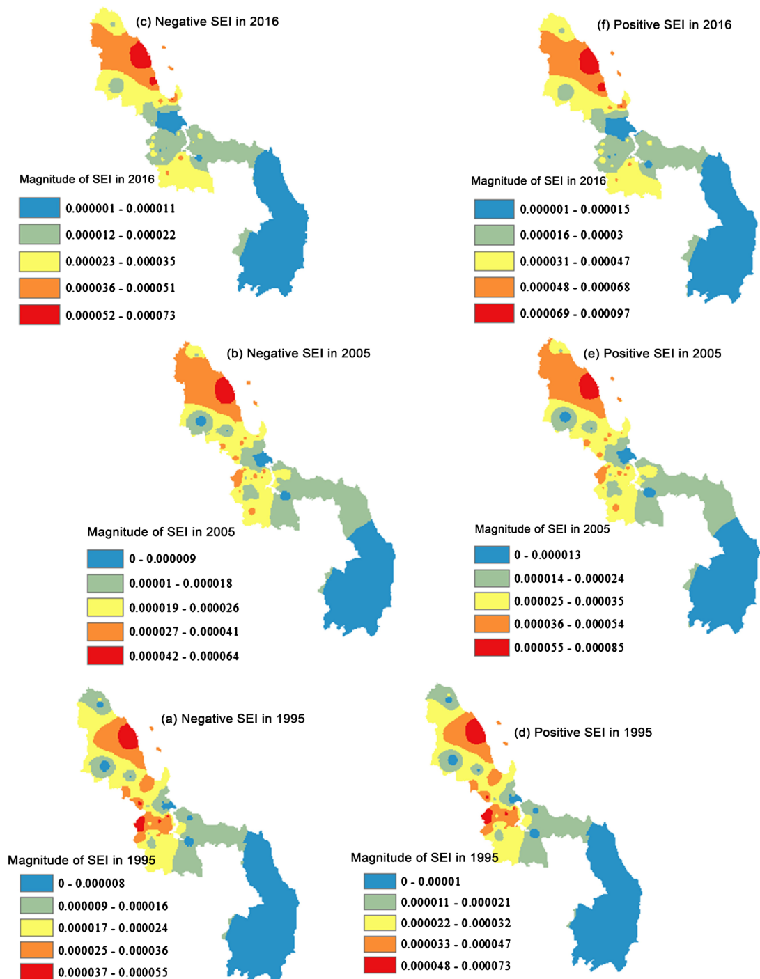
Figure 3. IDW spatial interpolation of BE impacts at Dar es Salaam Coastline.
