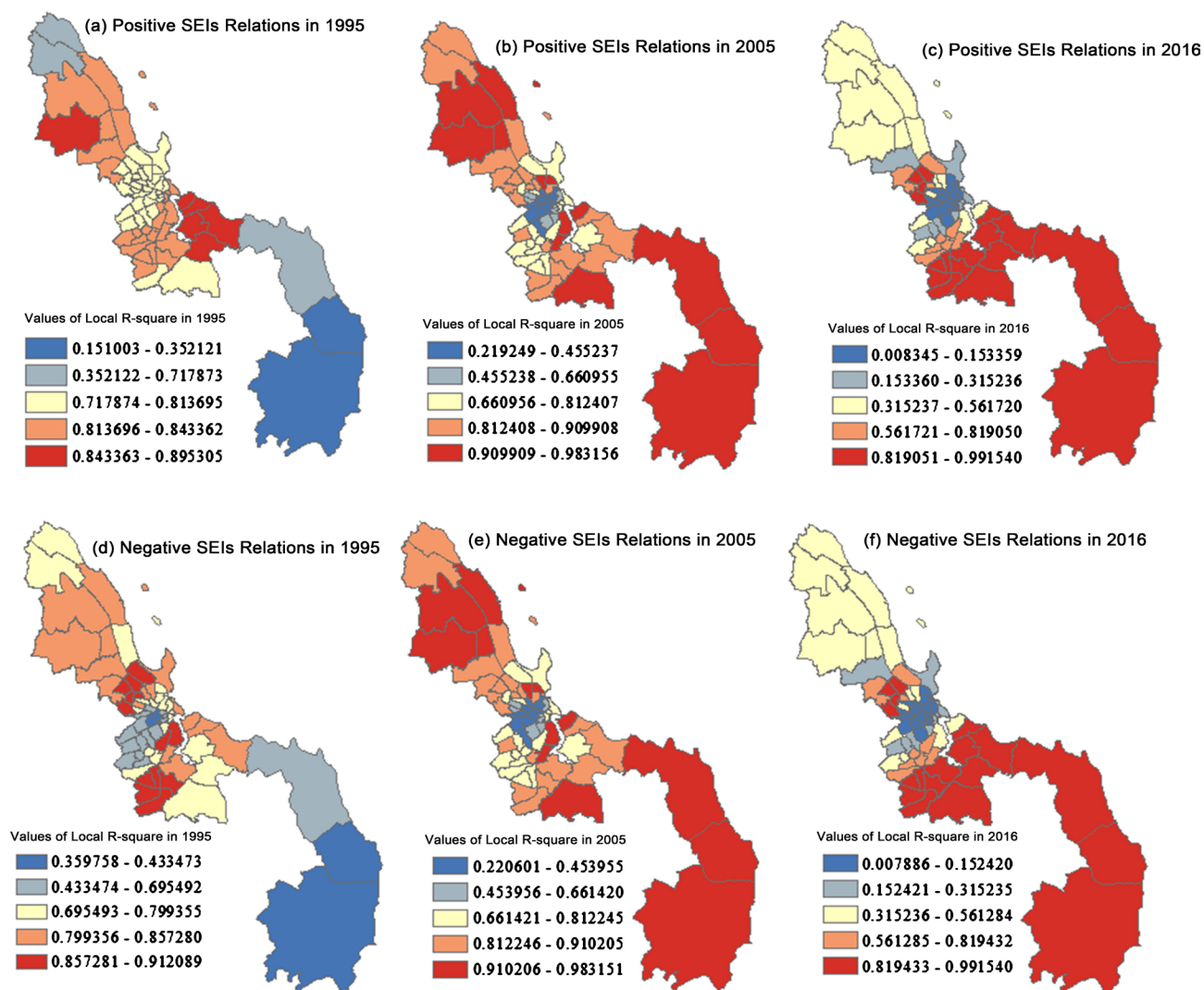
Figure 2. GWR analysis of positive and negative relationships in the study area.
